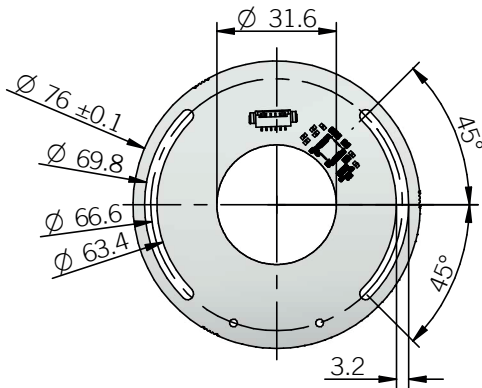
TARGET BOARD
