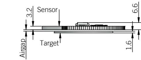
SENSOR BOARD
